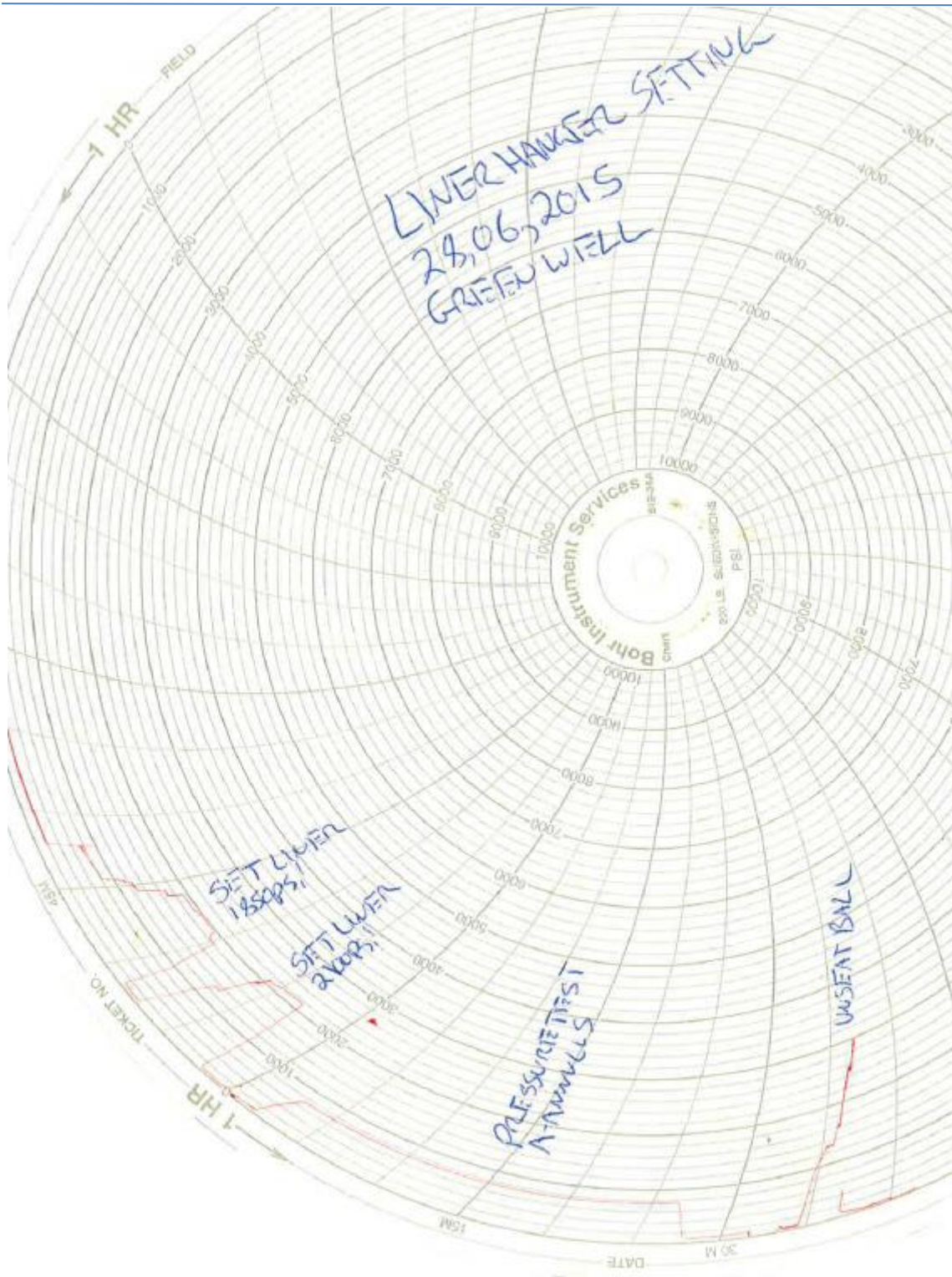
Figure 2: Test chart of Liner hanger packer pressure test to 50bar on 28-06-2015
